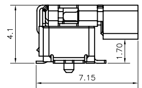
MATING VIEW
